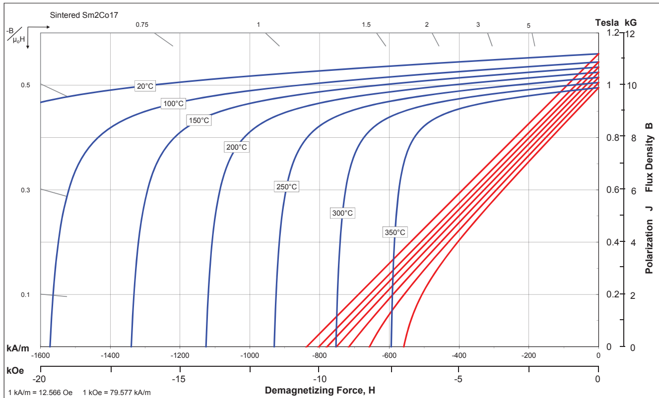
Demagnetization Curves
